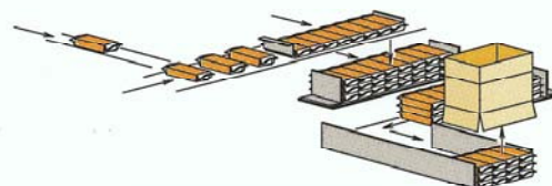
HIGH SPEED DOWNSTACKER / BOTTOM LOAD
